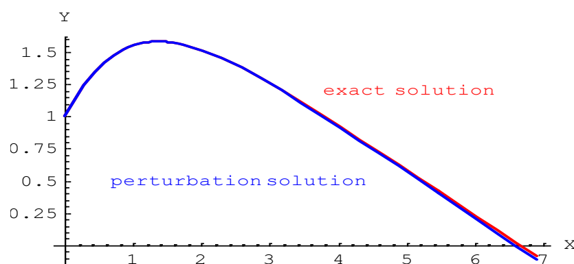
Fig. 4: A comparison of perturbation series approximations.
