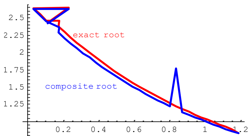
Fig. 2: Comparative solution draw for the proposed equation.
